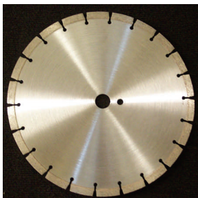
CS14DIYSEG12 14" SEGMENTED GENERAL PURPOSE 12MM SUPER DUTY WORK HORSE
